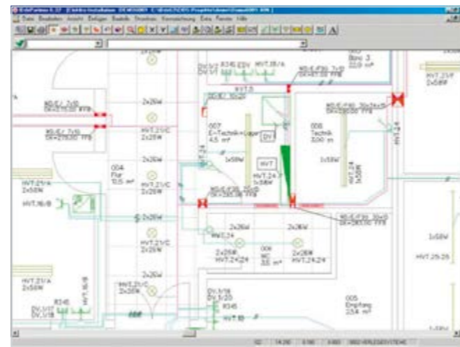
Installation plan 2-D/ 3-D
