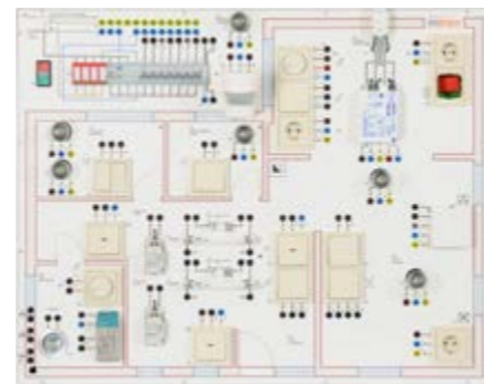
Lighting and appliance circuits
